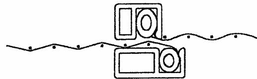
5 WICKET JAMB DETAIL SCALE: FULL
